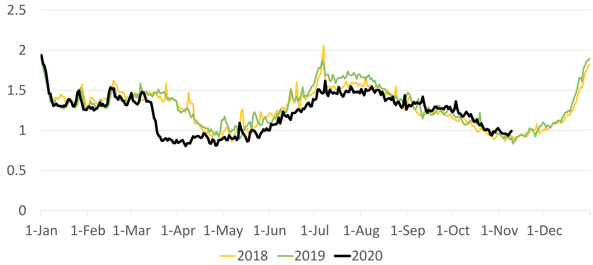
Influent Flow in Million Gallons per Day
