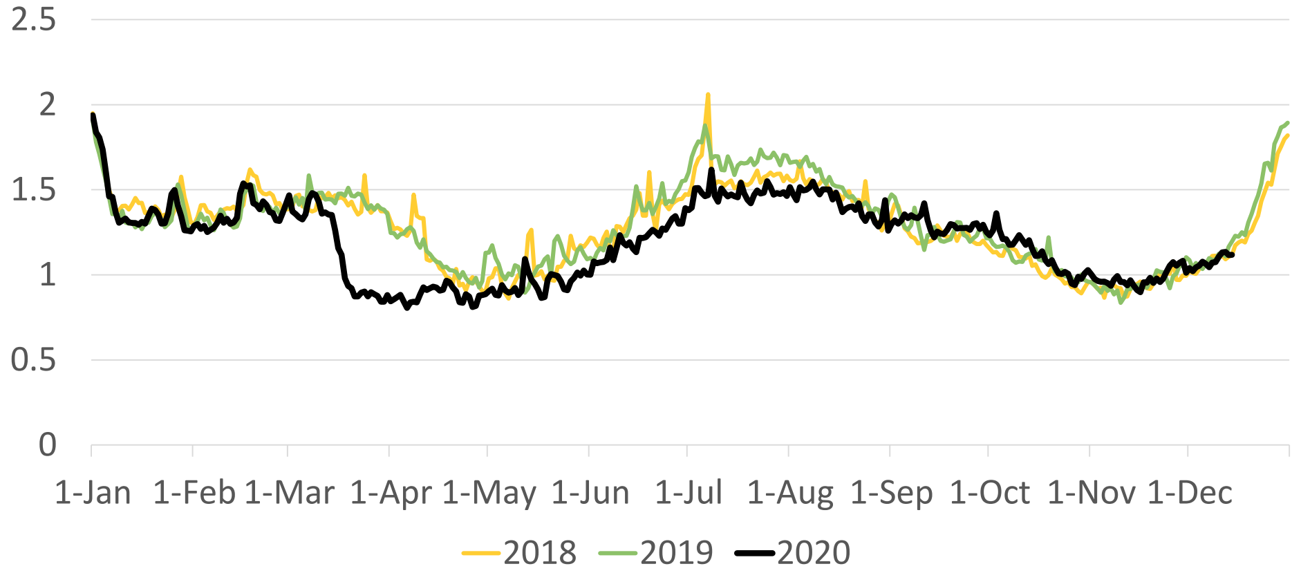
Influent Flow in Million Gallons per Day
