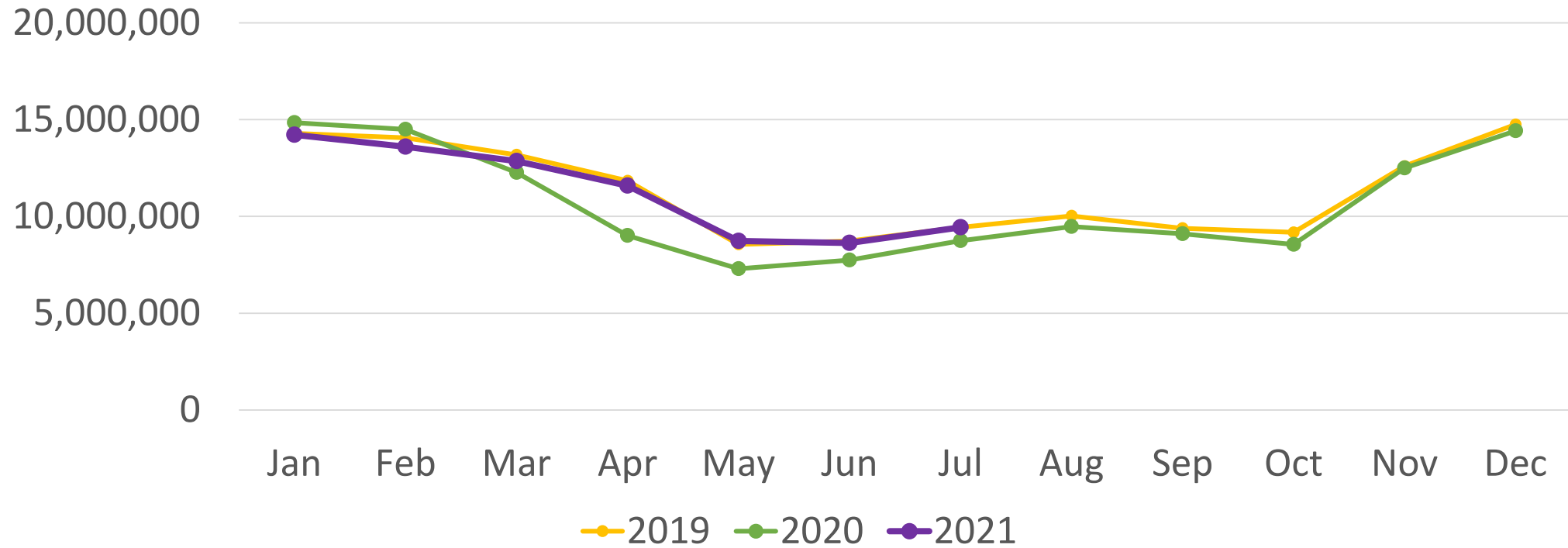
Pitkin County General Service kWhs Used
