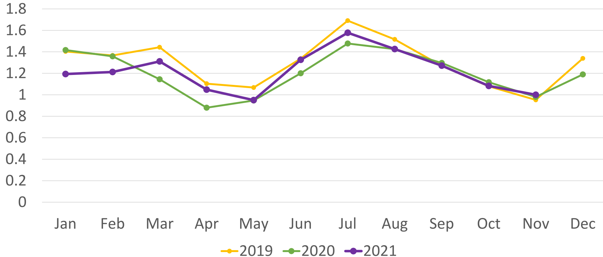
Influent Flow Gallons Per Day (Monthly Daily Average)
